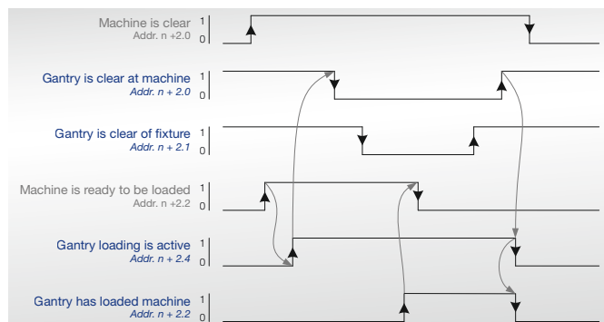
Signal-time diagram
