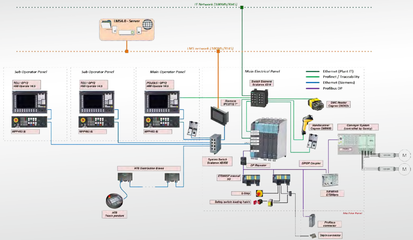
Control structure
