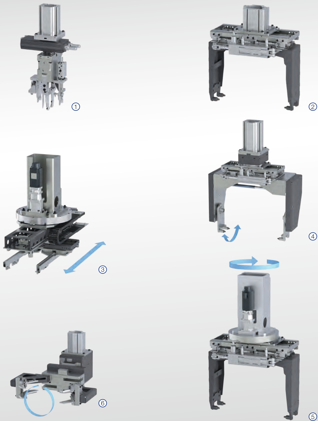
1 Crankshaft gripper · 2 Standard gripper for cubic parts · 3 Gripper for cubic parts with horizontal linear axis (Y-axis) · 4 Gripper for cubic parts with bucket axis (A-axis) · 5 Gripper for cubic parts with rotary axis (C-axis) · 6 Gripper for cubic parts with rotation axis (D-axis)
